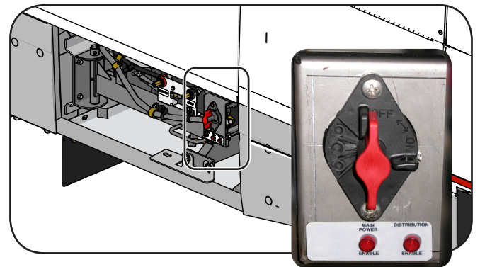
Figure 4 - 12/24V battery disconnect switch
