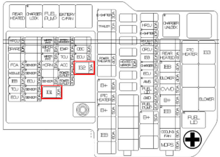
Engine room fuse box
