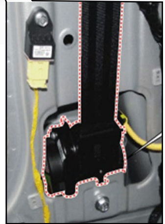
1. Front Seatbelt Pretensioner
