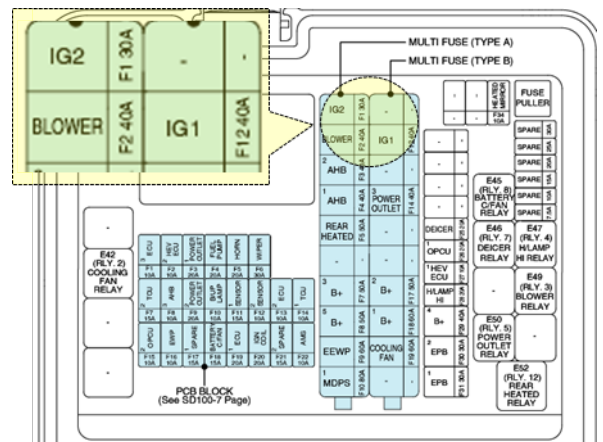
Engine room fuse box
